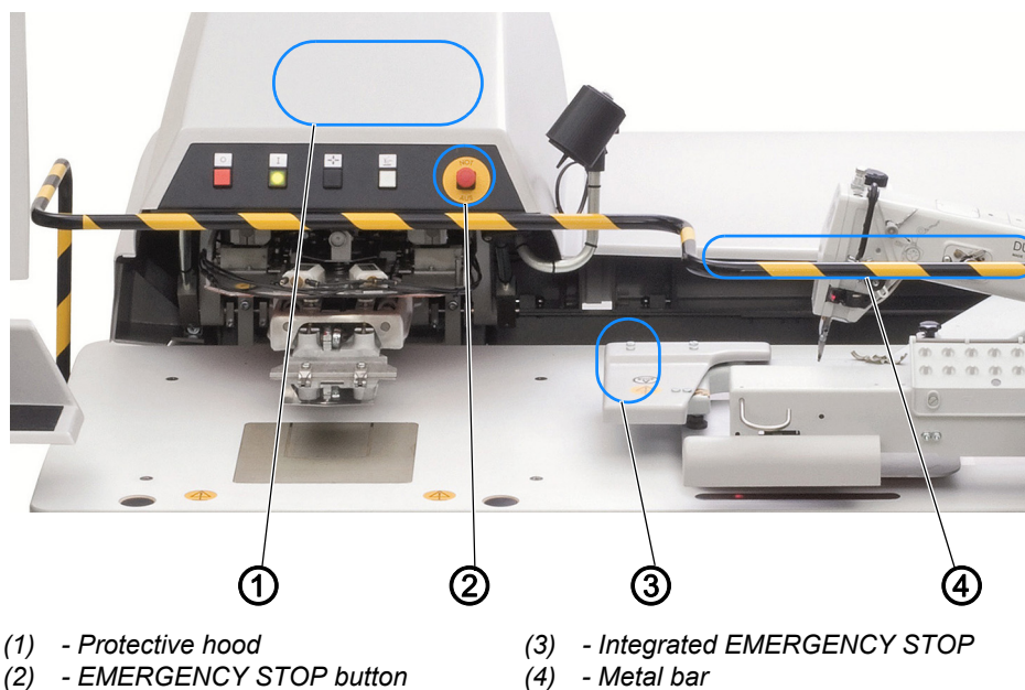
Fig. 1: Safety equipment
