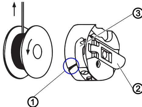
Fig. 19: Changing the hook thread bobbin (806N-121-10)
