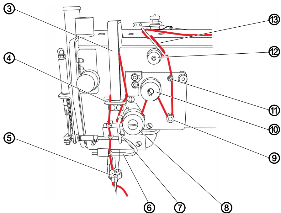
Fig. 14: Threading the needle thread (806N-111-10) (2)
