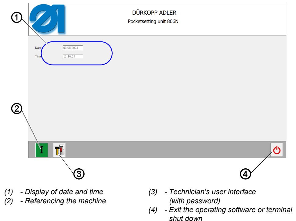
Fig. 51: Start screen
