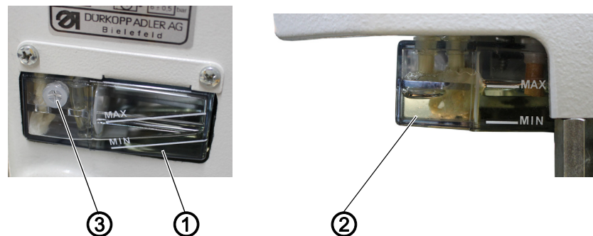
Fig. 75: Lubricating (806N-121-10) (2)
