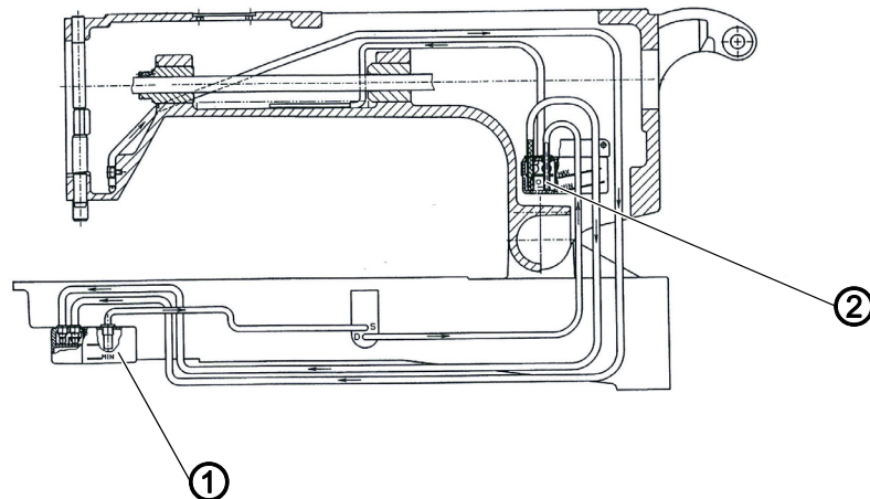
Fig. 74: Lubricating (806N-121-10) (1)
