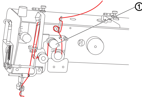
Fig. 24: Setting the needle thread tension (806N-111-10)
