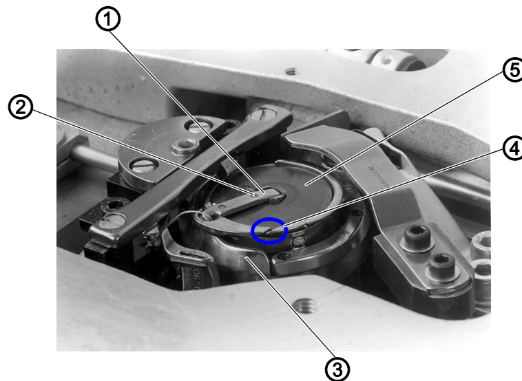
Fig. 20: Changing the hook thread bobbin (806N-111-10)
