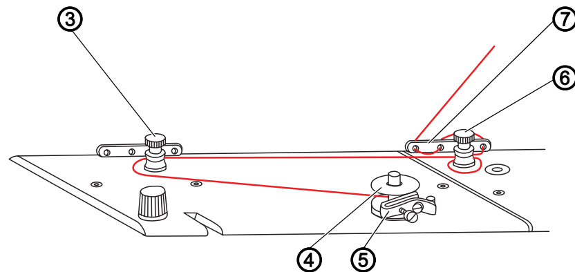
Fig. 18: Winding the bobbin thread (806N-111-10) (2)
