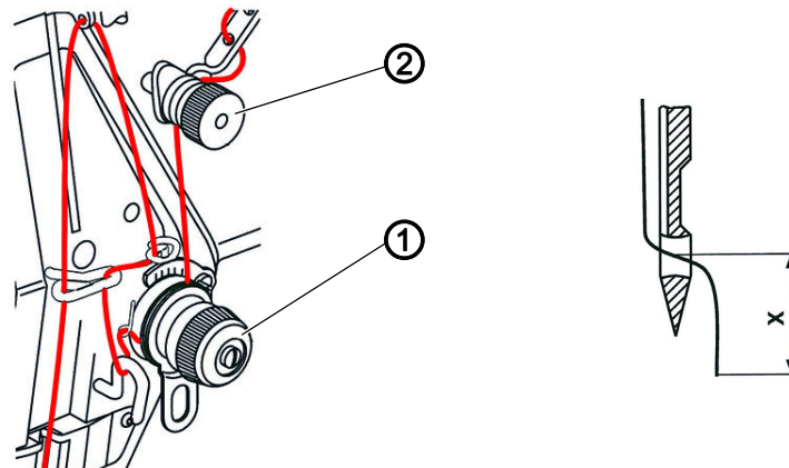
Fig. 23: Setting the needle thread tension (806N-121-10)
