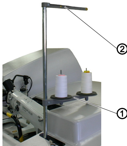
Fig. 15: Winding the bobbin thread (806N-121-10) (1)
