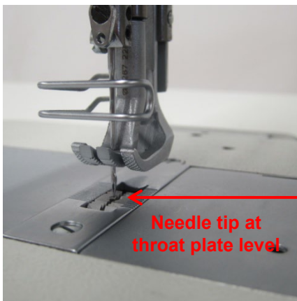
Fig. 6: Needle position
